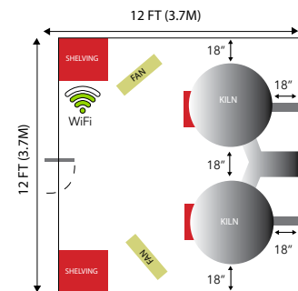
Typical layout for a dual kiln studio.
