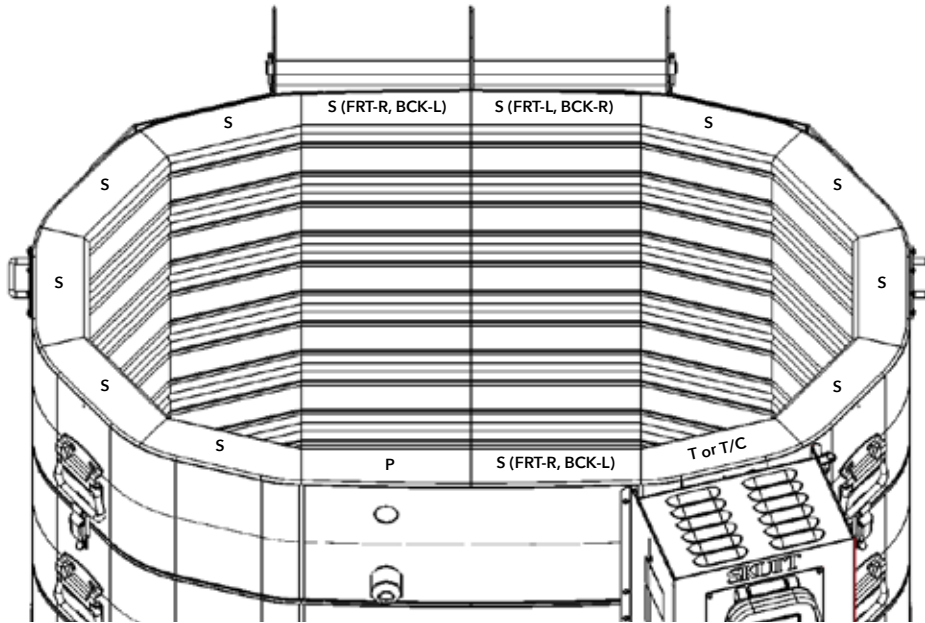
1427-3" PK BRICK DIAGRAM
